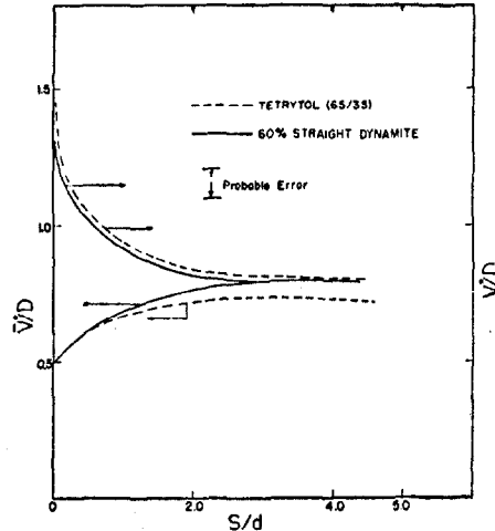
Fig 4 Shock velocity V^* versus S and average velocity V_1^* versus S for propagation by influence in air for a straight dynamite and 65/35 tetrytol
